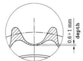
Induction hardened teeth HRC 45±3
